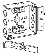
52151 MS X* MS bracket for 1/4", 2 1/2", 3/4", 4" metal studs
