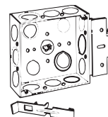
52151 MS 1/2 & 3/4 For use on 1", 2", 3", 4" studs
