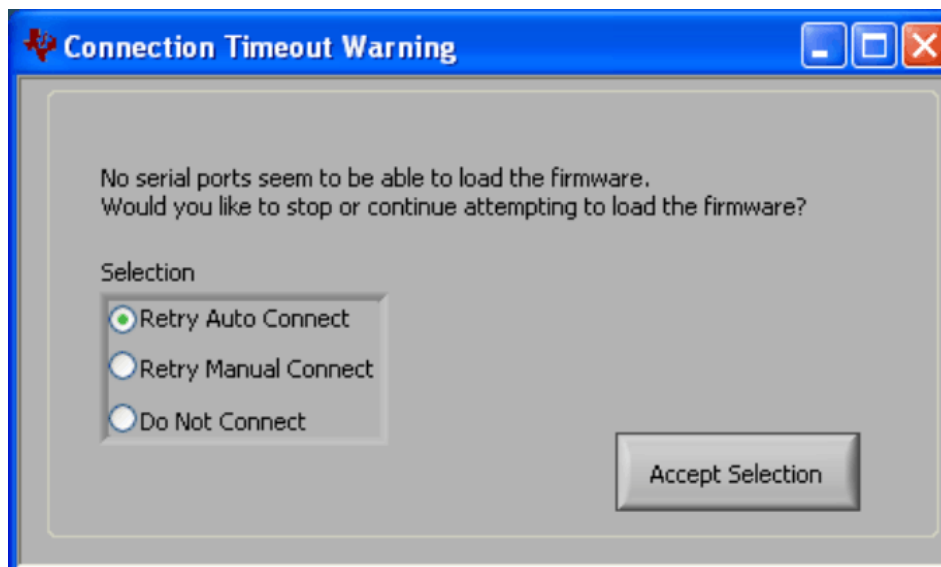
Figure 9. Connection Timeout
