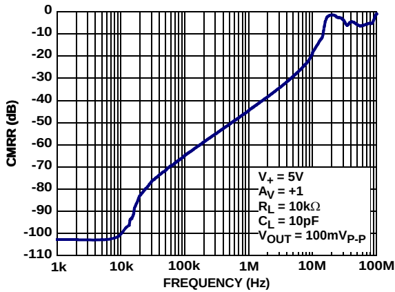
FIGURE 7. CMRR vs FREQUENCY
