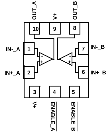
ISL28290 (10 Ld \mu TQFN) TOP VIEW
