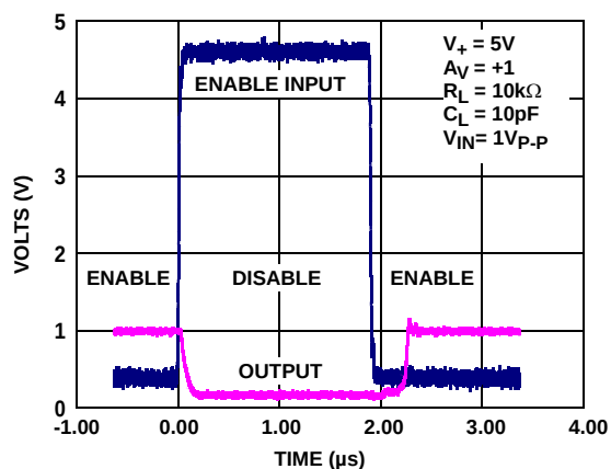
FIGURE 13. ENABLE/DISABLE TIMING
