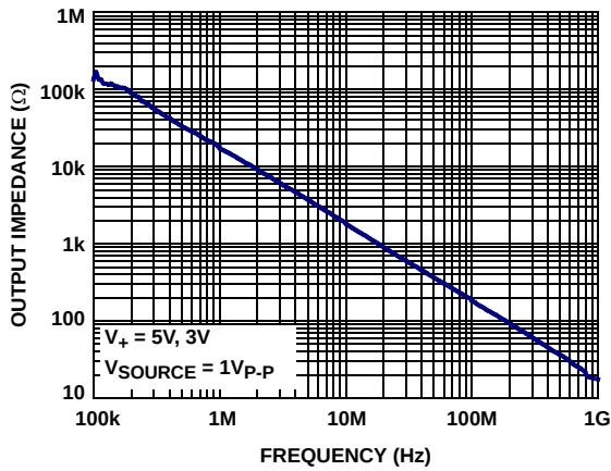
FIGURE 5. DISABLED OUTPUT IMPEDANCE vs FREQUENCY
