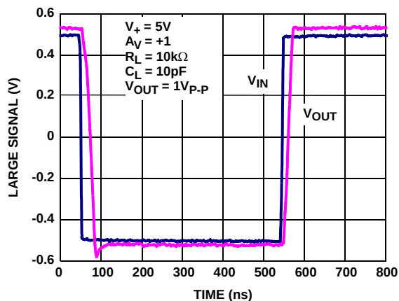
FIGURE 15. LARGE SIGNAL STEP RESPONSE RISE AND FALL TIME
