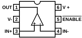
ISL28190 (6 LD SOT-23) TOP VIEW
