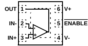
ISL28190 (6 LD 1.6X1.6X0.5 \mu TDFN) TOP VIEW
