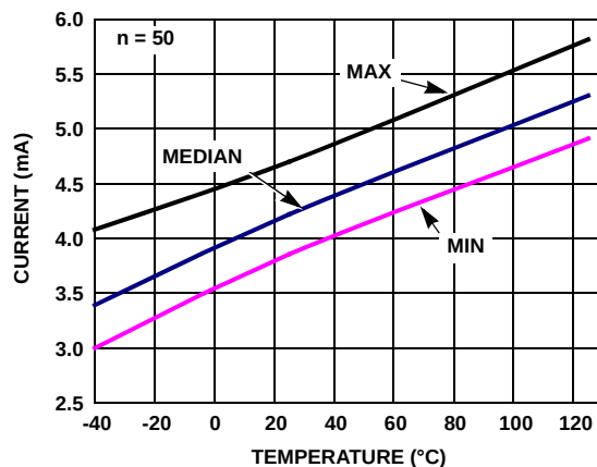
FIGURE 16. SUPPLY CURRENT vs TEMPERATURE V_S = \pm 2.5V ENABLED. R_L = \text{INF}
