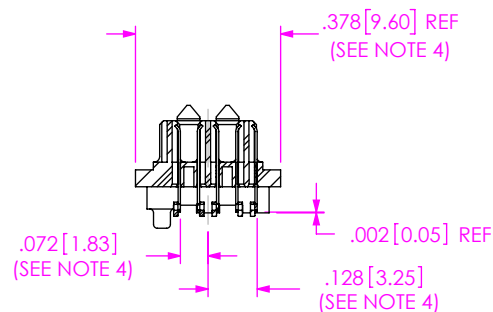
FIG 7 -05: 5 ROWS (SEAM-20-03.5-XXX-05-1-A SHOWN) (SAME AS FIG 6, EXCEPT AS SHOWN) (SOME CENTER FEATURES REMOVED FOR CLARITY) (SEE NOTE 4)
