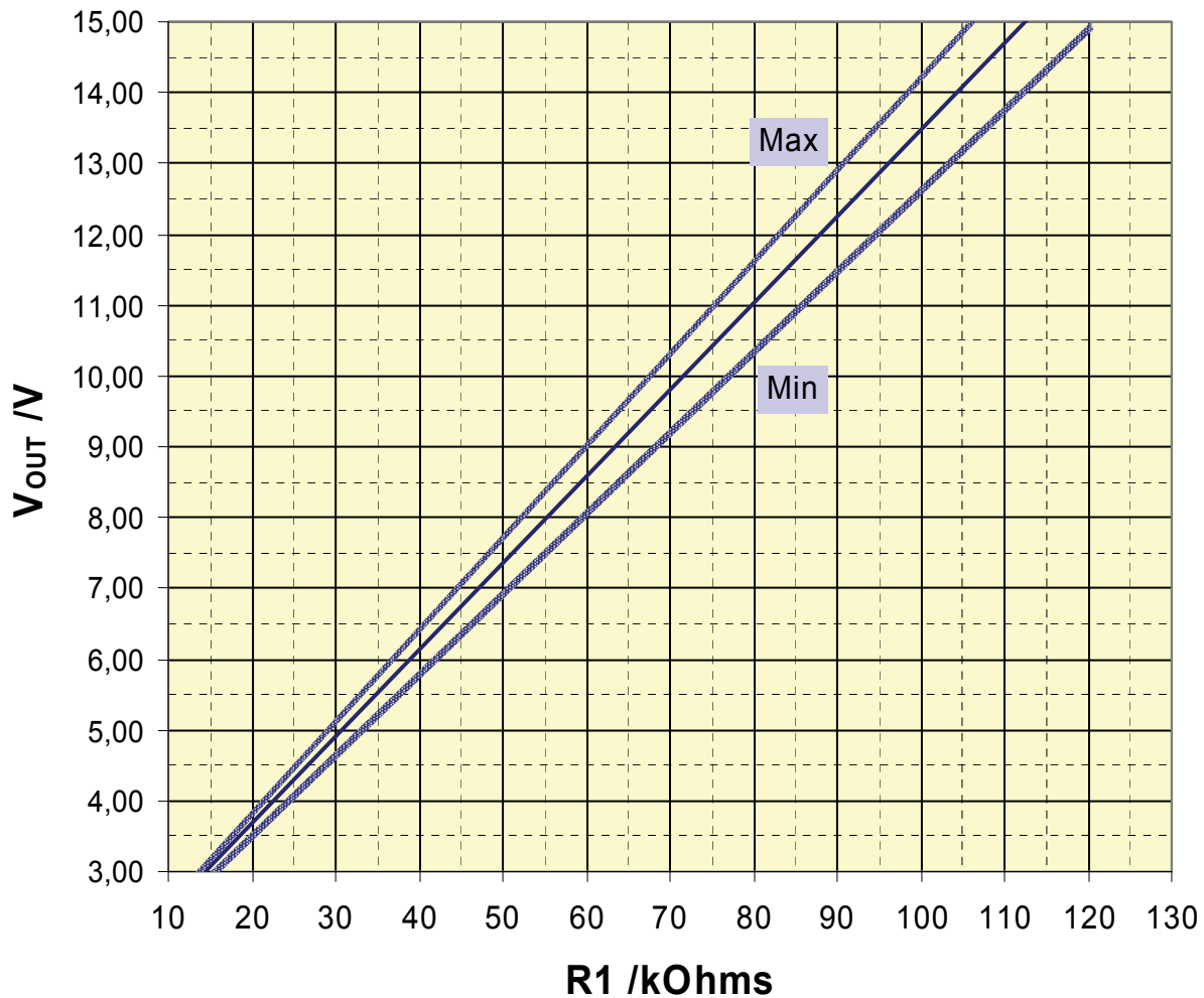
Figure 3.22 DC/DC Converter Output Voltage as Function of R1 (R2 = 10kOhms)
