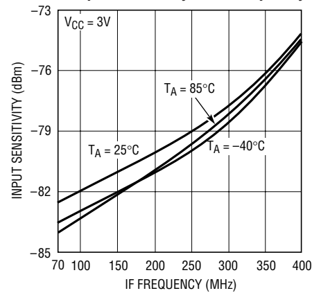
IF Input Sensitivity vs IF Frequency
