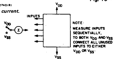
Fig. 11 - Input current.
