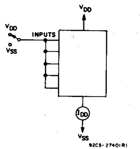
Fig. 9 - Quiescent device current.
