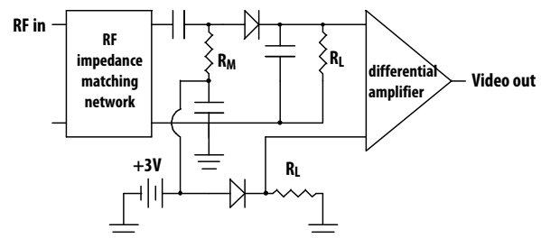
Figure 13. Differential Detector.
