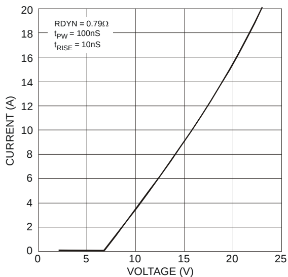
Figure 9 4 TLP, t_{PW} = 100\text{nS} , t_{RISE} = 10\text{nS} Data to GND
