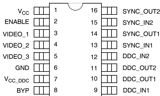
16 Pin QSOP
