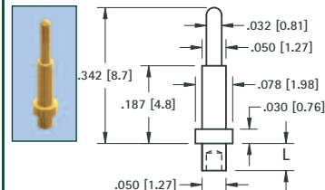
.032 (.81) PIN - SWAGE MOUNT
