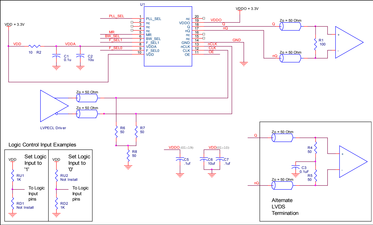
Figure 5. ICS874001I-02 Schematic Layout
