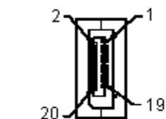
Conn1: Display Port 20P M
