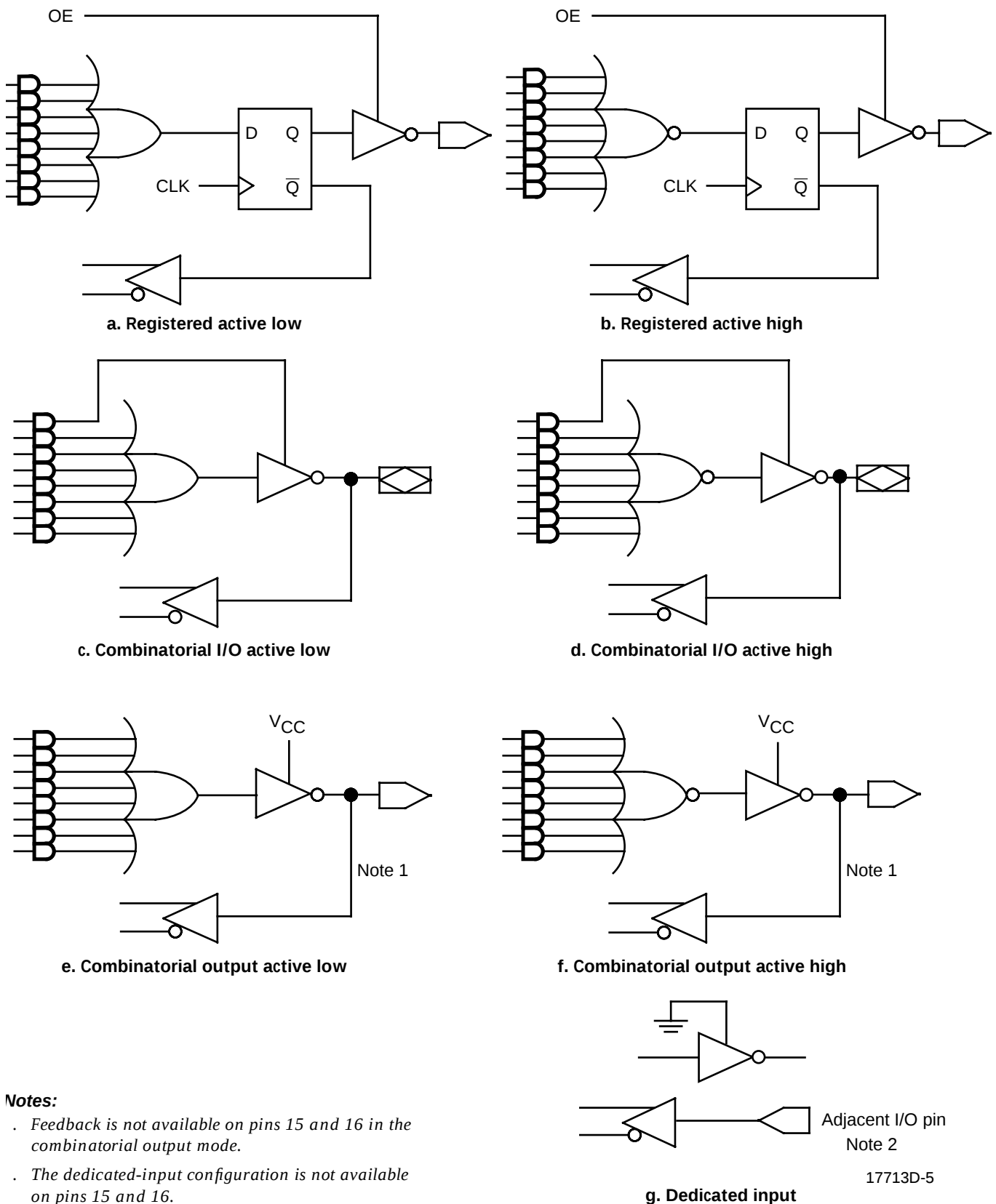
Figure 2. Macrocell Configurations
