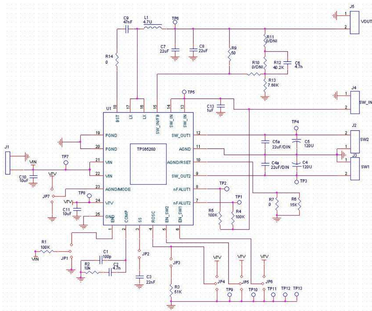
Figure 7. TPS65280EVM Schematic
