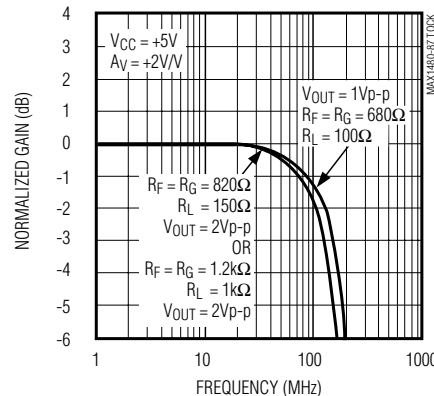
MAX4180 LARGE-SIGNAL GAIN vs. FREQUENCY (SINGLE SUPPLY)
