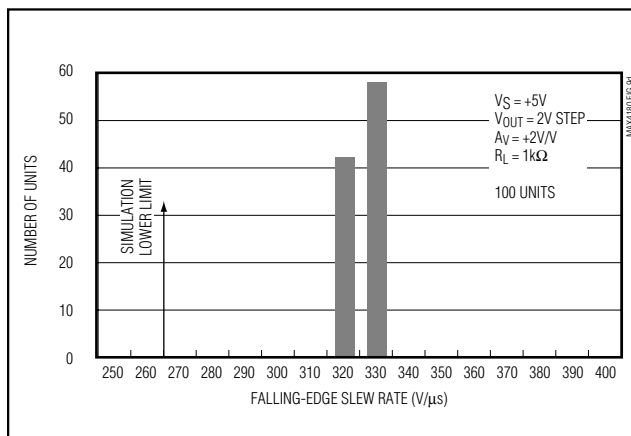
Figure 9d. MAX4180 Falling-Edge Slew-Rate Distribution (Single Supply)
