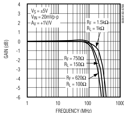
MAX4184/MAX4185 SMALL-SIGNAL GAIN vs. FREQUENCY (DUAL SUPPLIES)
