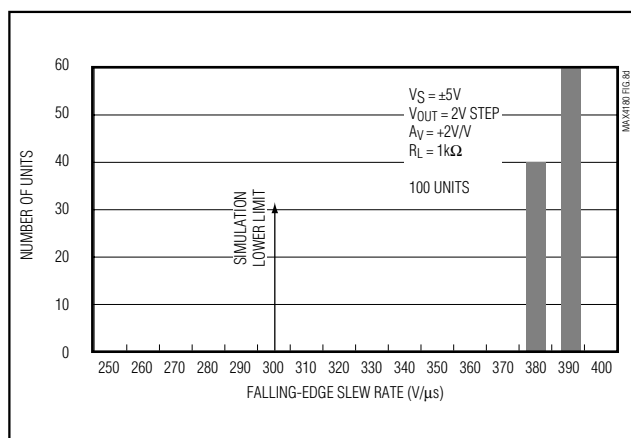
Figure 8d. MAX4180 Falling-Edge Slew-Rate Distribution (Dual Supplies)
