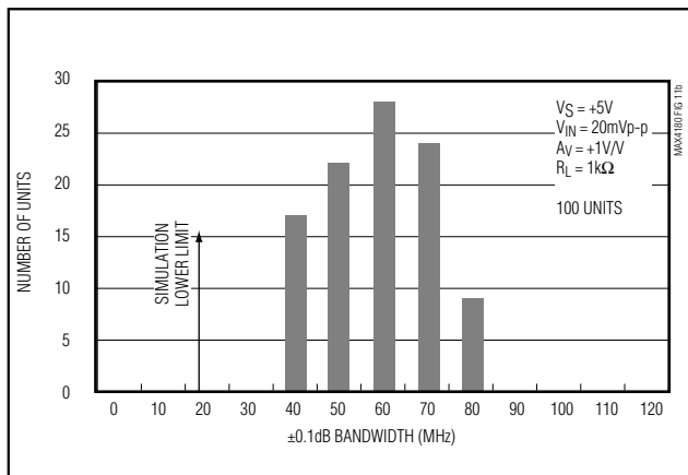
Figure 11b. MAX4181 \pm 0.1dB Bandwidth Distribution (Single Supply)
