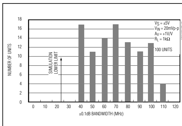
Figure 10b. MAX4181 ±0.1dB Bandwidth Distribution (Dual Supplies)
