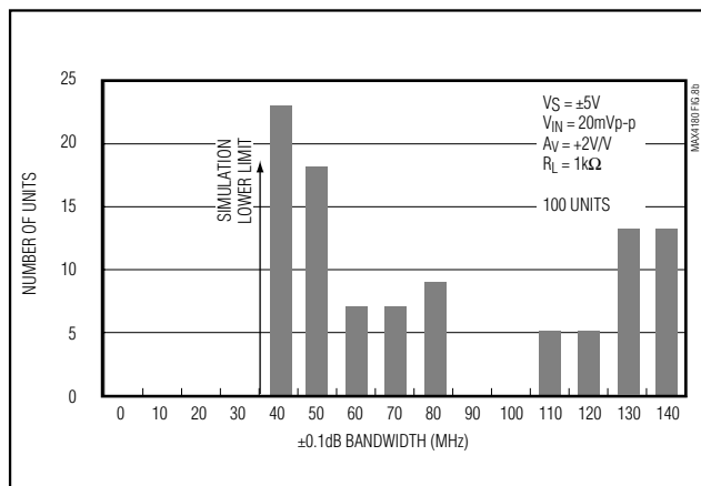
Figure 8b. MAX4180 \pm 0.1 dB Bandwidth Distribution (Dual Supplies)
