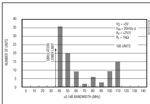
Figure 9b. MAX4180 \pm 0.1 dB Bandwidth Distribution (Single Supply)
