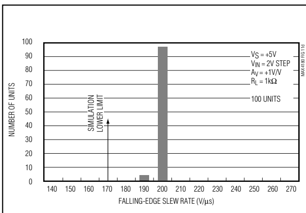
Figure 11d. MAX4181 Falling-Edge Slew-Rate Distribution (Single Supply)
