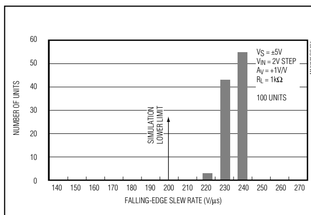
Figure 10d. MAX4181 Falling-Edge Slew-Rate Distribution (Dual Supplies)
