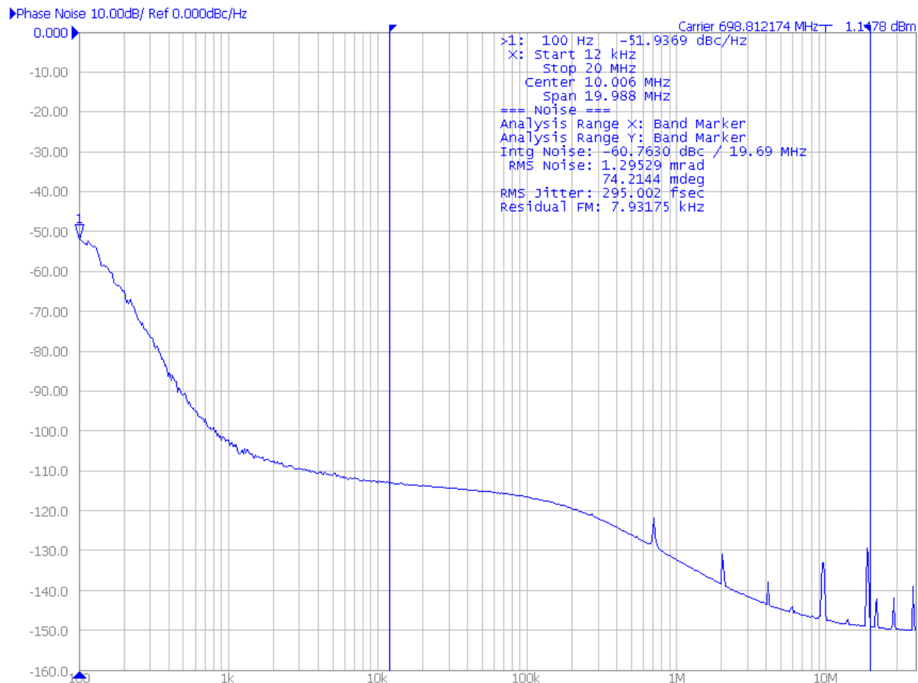
Figure 3. Typical Phase Noise Plot
