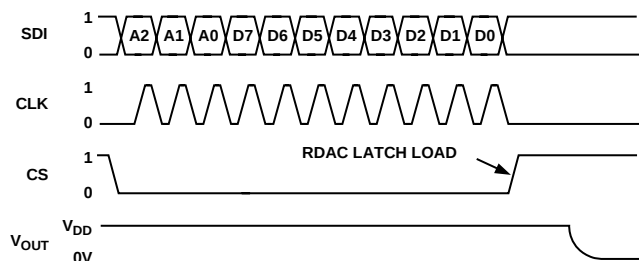
Figure 1. Timing Diagram
