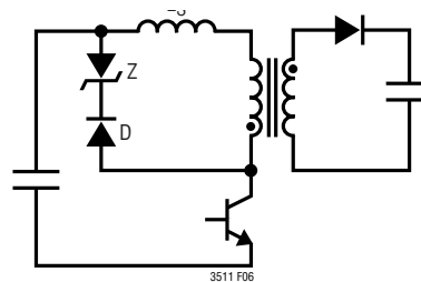
Figure 6. DZ Clamp
