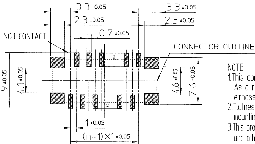
RECOMMENDED PC BOARD LAYOUT (COMPONENT SIDE)
