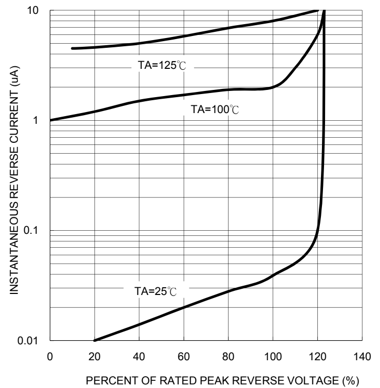
FIG. 2- TYPICAL REVERSE CHARACTERISTICS
