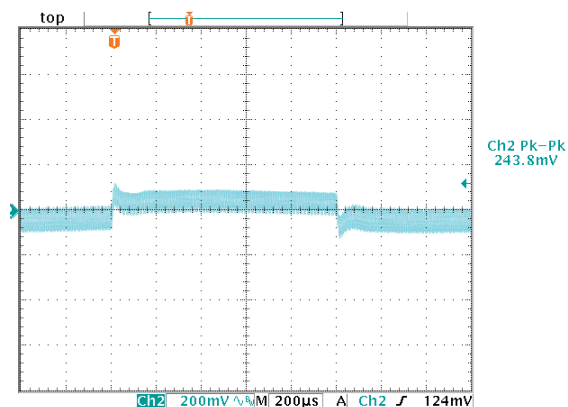
Transient Response (Load 50% to 75%, 470μF electrolytic cap and 1μF ceramic cap)
