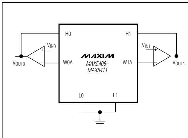
Figure 6. Gain Control
