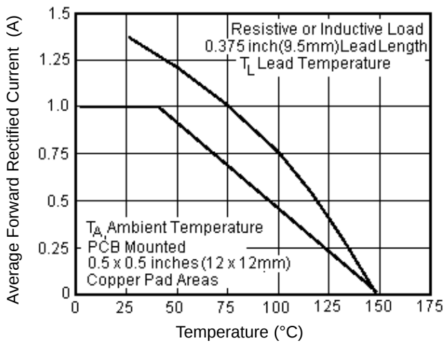
Forward Current Derating Curves
