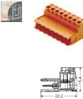
Pin plugs SLS 5.08/180B
