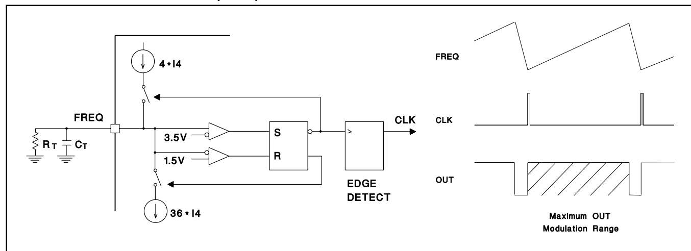
Figure 3. Clock generator.
