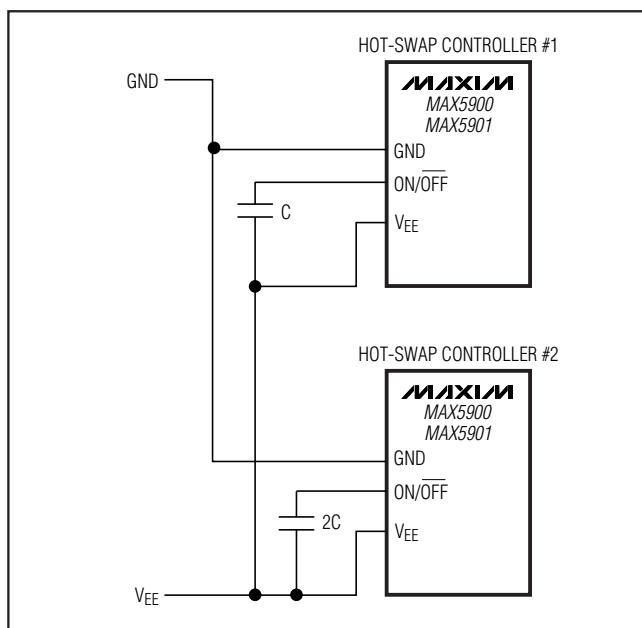
Figure 3. Power-Supply Sequencing
