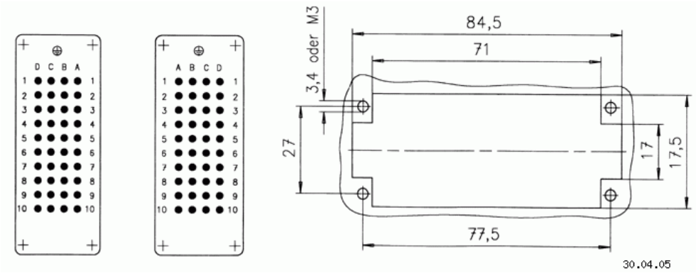
Contact arrangement
