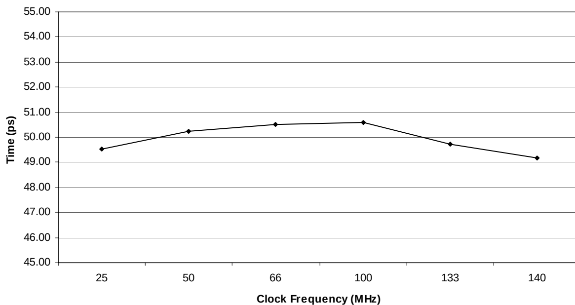
Output Duty Cycle vs Clock Frequency A_{VDD} and V_{DD} = 3.3V T_a = 25^\circ C
