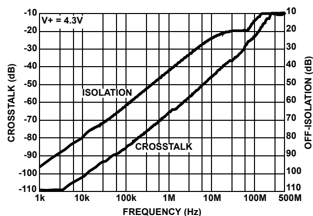
FIGURE 23. CROSSTALK AND OFF-ISOLATION
