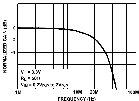
FIGURE 22. FREQUENCY RESPONSE
