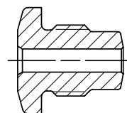
122178 DRIVING ANVIL -06 POP RIVET
