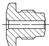
122177 DRIVING ANVIL -05 POP RIVET
