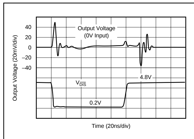
FIGURE 12. Disable/Enable Glitch.
