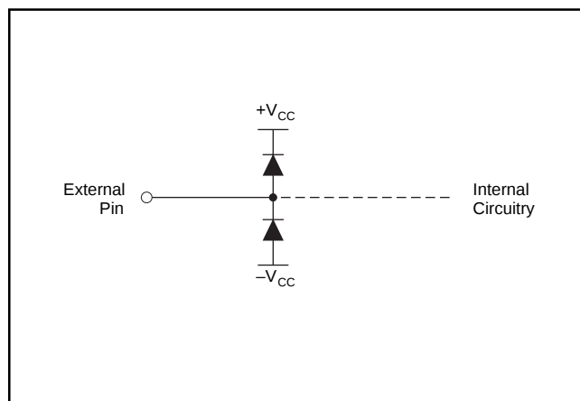
FIGURE 13. Internal ESD Protection.
