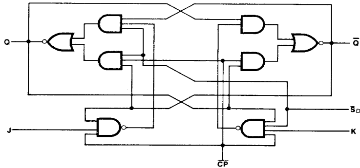
LOGIC DIAGRAM (one half shown)
