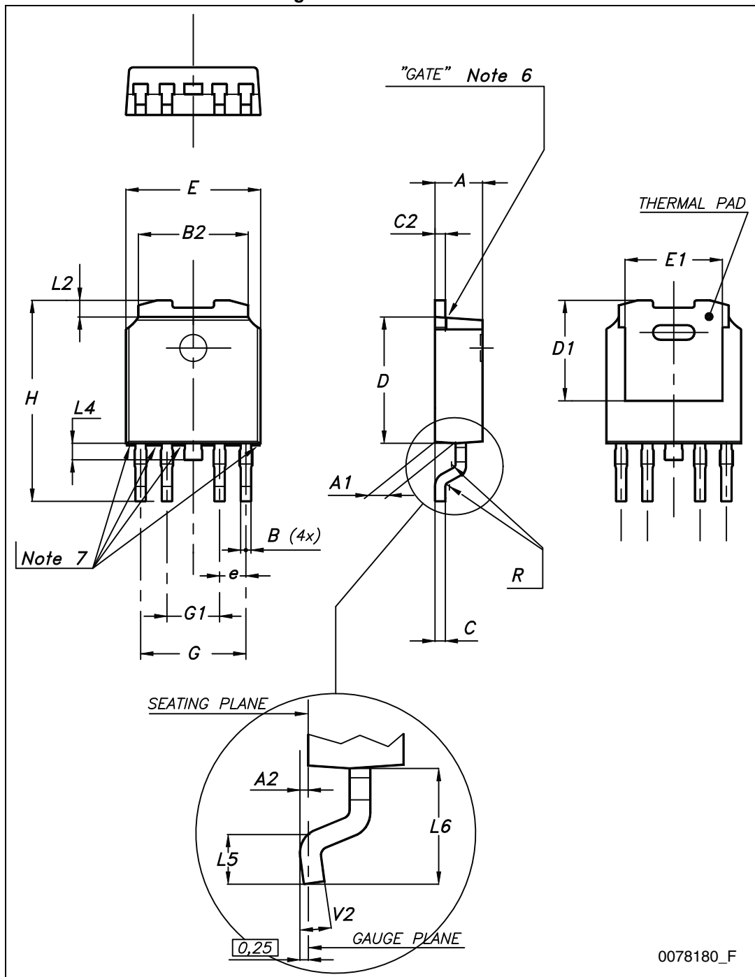
Figure 25. PPAK outline
