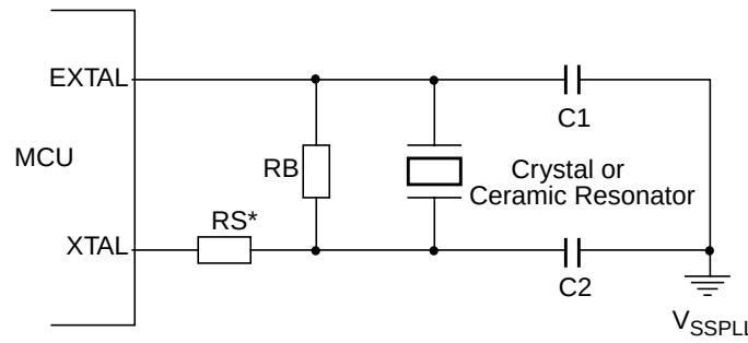
Figure 3-3. Full Swing Pierce Oscillator Connections ( \overline{\text{XCLKS}} = 0 )
