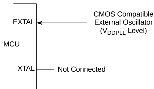
Figure 3-4. External Clock Connections ( \overline{\text{XCLKS}} = 0 )
