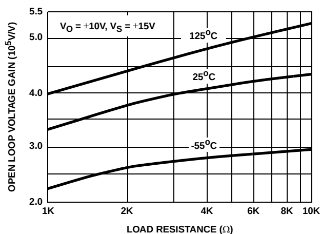
FIGURE 15. A_{VOL} vs LOAD RESISTANCE
