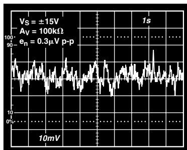
TPC 32. 0.1 Hz to 10 Hz Noise
