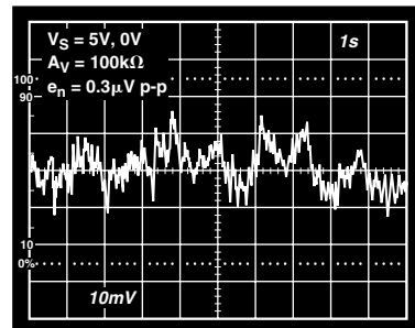
TPC 33. 0.1 Hz to 10 Hz Noise
