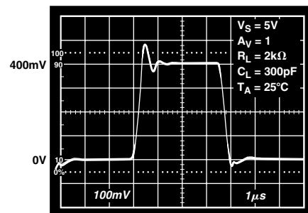
TPC 36. Small Signal Transient Response
