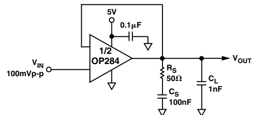
Figure 16. Snubber Network Compensates for Capacitive Load
