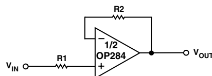
Figure 7. A Resistance in Series with an Input Limits Overvoltage Currents to Safe Values
