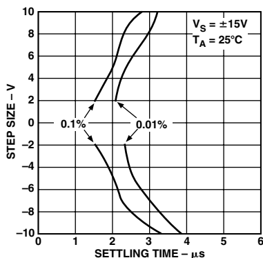
TPC 31. Settling Time vs. Step Size
