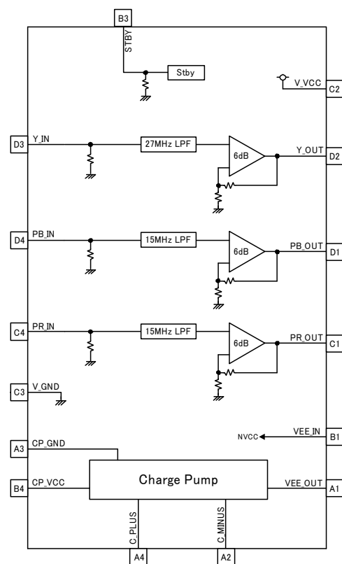
Fig.2. Block diagram
