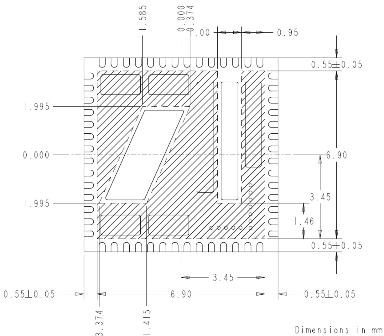
Figure 13: EN6382QI Package – PCB Footprint Keepout (Bottom view)
