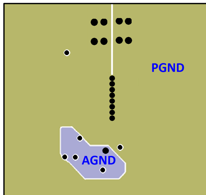
Figure 9: Inner Layer 2 – grounds
