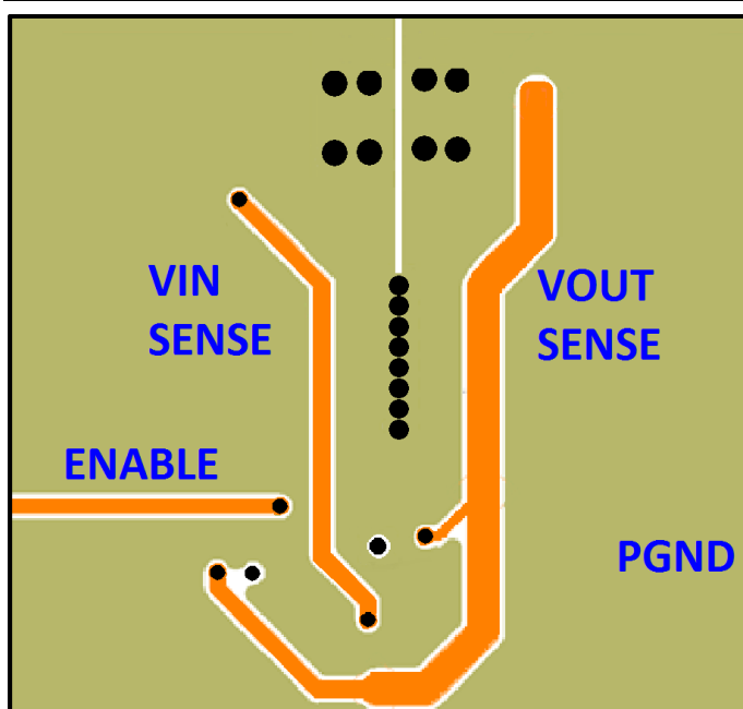
Figure 10: Inner Layer 3 – routing
