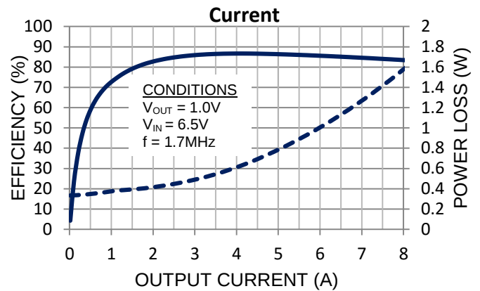
Efficiency, Power Loss vs Output Current
