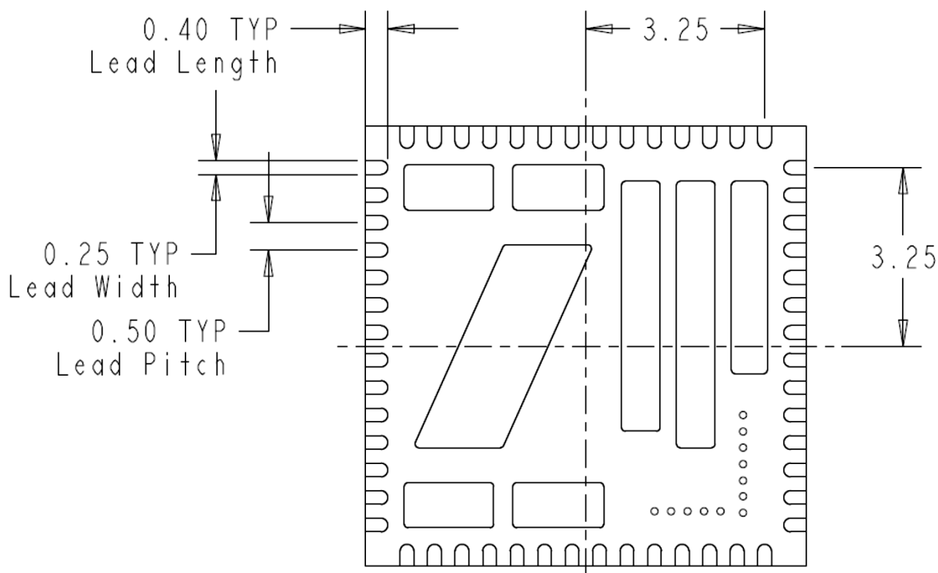
Figure 12: Lead-Frame exposed metal (Bottom View)
