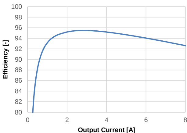
Figure 6: Efficiency V_{IN} = 5.5V , V_{OUT} = 3.3V
