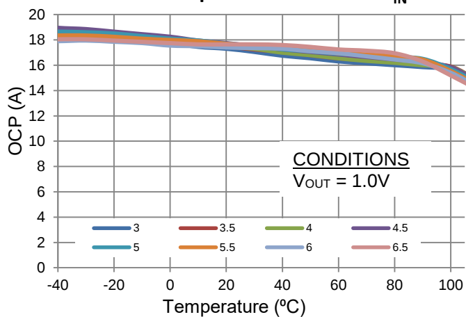
OCP vs Temperature at various V_{IN}
