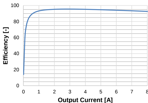
Figure 2: Efficiency at V_{IN} = 5V , V_{OUT} = 3.3V
