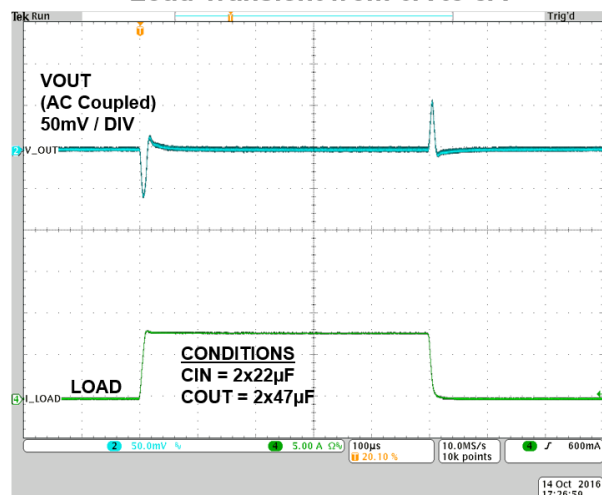
Load Transient from 0A to 8A
