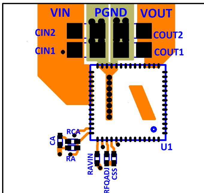
Figure 8: Top Layout with Critical Components Only (Top View). See Figure 7 for corresponding schematic.
