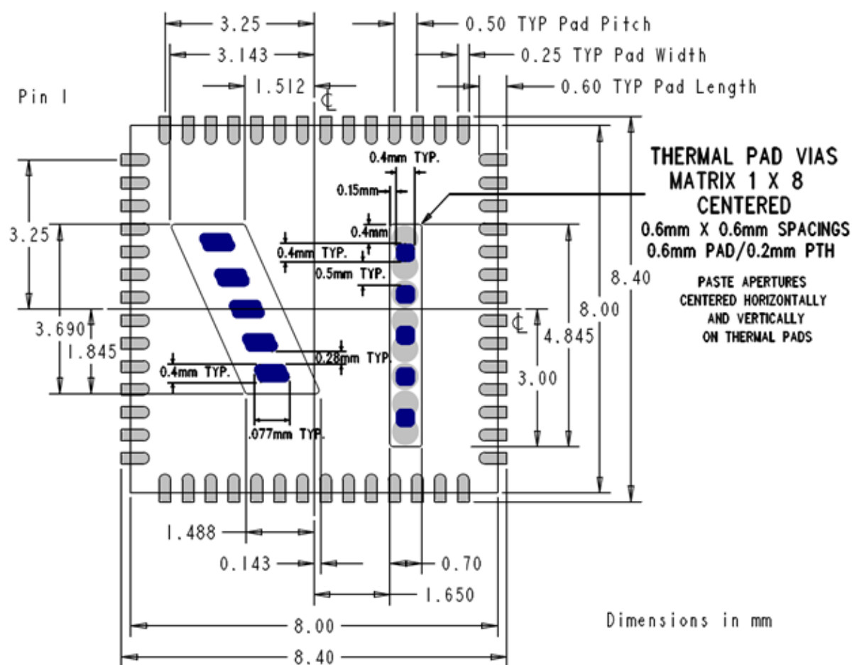
Figure 14: Solder stencil drawing (Top View)
