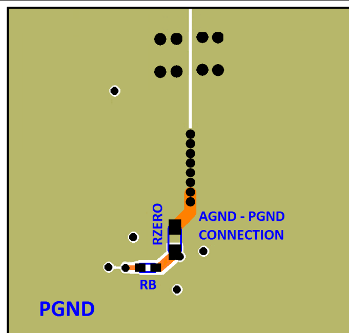
Figure 11: Bottom Layer – components
