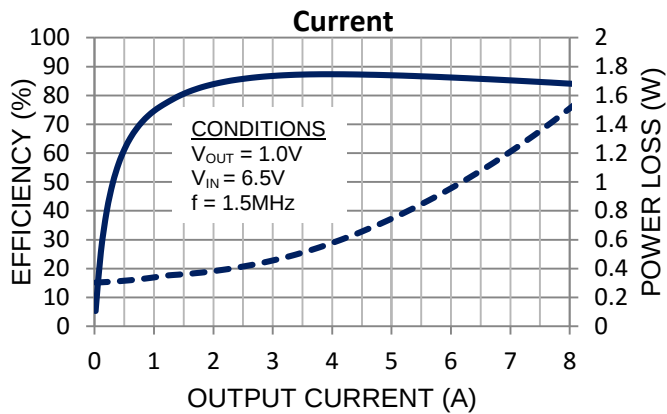
Efficiency, Power Loss vs Output Current
