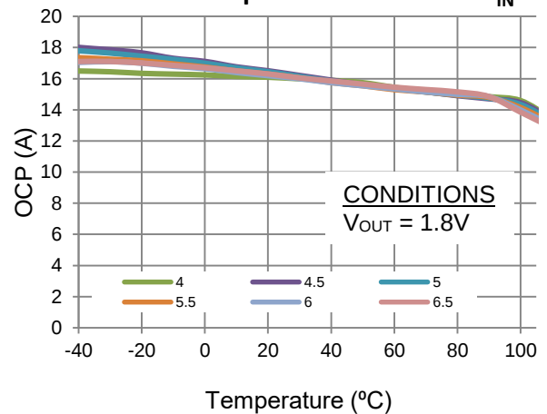
OCP vs Temperature at various V_{IN}
