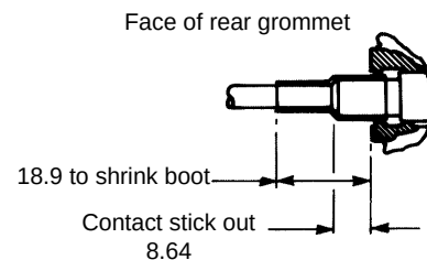
M39029/90/91A in situ dimensions
