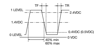
Figure 2) TTL Output Wave Form
