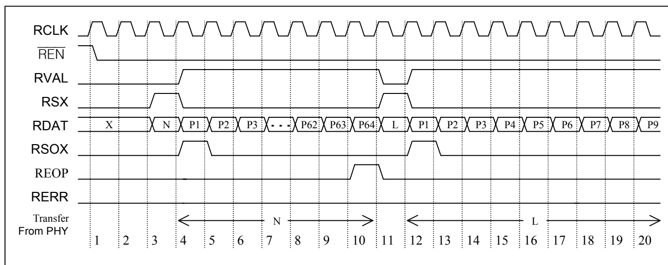
Figure 8-30. POS-PHY Level 3 Receive Multiple Packet Transfer In-Band Addressing
