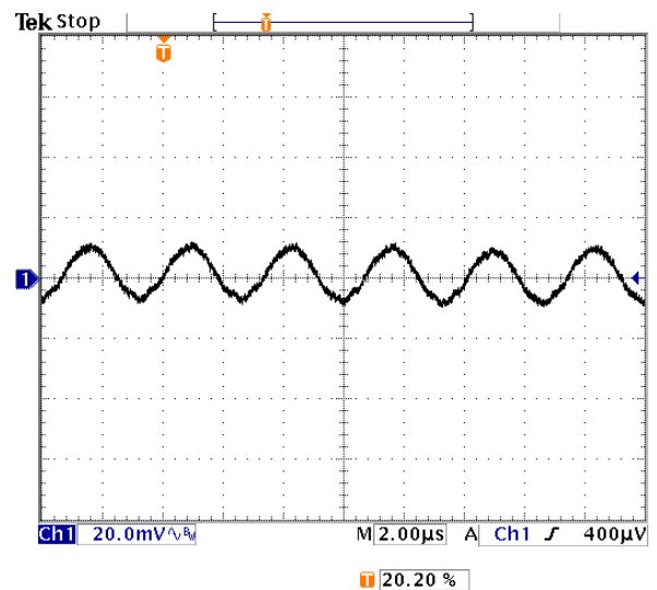
Fig-1.2V-5: Output voltage ripple (20mV/div.) for Vout=1.2V at full rated load current into a resistive load with external capacitance 47 \mu Fx4 ceramic + 1 \mu F ceramic at Vin=5.0V.
