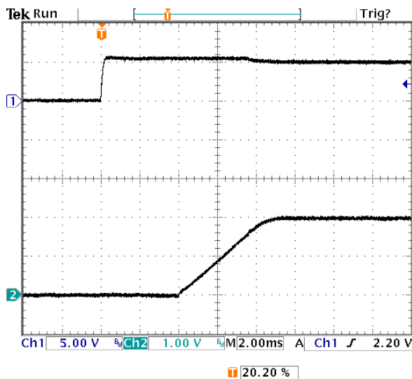
Fig-2.0V-4: Turn-on transient for Vout=2.0V with application of Vin at full rated load current (resistive) and 47 \mu Fx4 external capacitance at Vin=5.0V.
