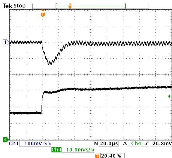
Fig-1.2V-6: Output voltage response for Vout=1.2V to positive load current step-change from 8A to 16A with slew rate of 5A/ \mu s at Vin=5.0V. Co=47 \mu Fx4 ceramic.
