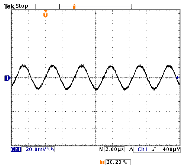
Fig-2.0V-5: Output voltage ripple (20mV/div.) for Vout=2.0V at full rated load current into a resistive load with external capacitance 47 \mu Fx4 ceramic + 1 \mu F ceramic at Vin=5.0V.
