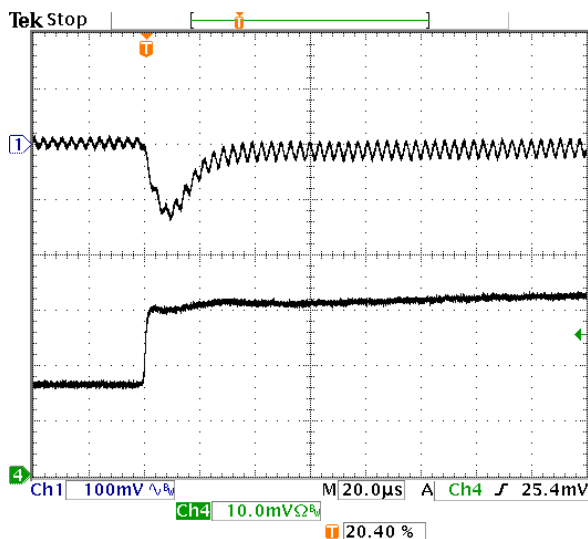
Fig-2.0V-6: Output voltage response for Vout=2.0V to positive load current step-change from 8A to 16A with slew rate of 5A/ \mu s at Vin=5.0V. Co=47 \mu Fx4 ceramic.
