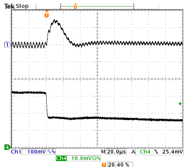
Fig-2.0V-7: Output voltage response for Vout=2.0V to positive load current step-change from 16A to 8A with slew rate of -5A/ \mu s at Vin=5.0V. Co=47 \mu Fx4 ceramic.
