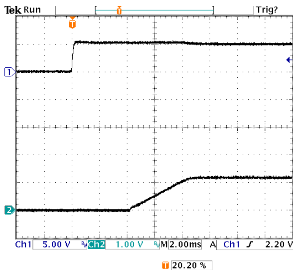
Fig-1.2V-4: Turn-on transient for Vout=1.2V with application of Vin at full rated load current (resistive) and 47 \mu Fx4 external capacitance at Vin=5.0V.
