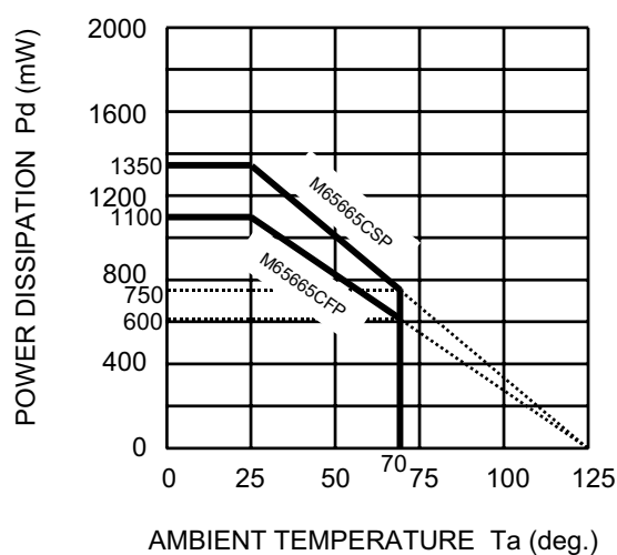
THERMAL DERATING (MAXIMUM RATING)
