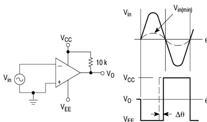
Figure 7. Zero Crossing Detector (Split Supplies)
