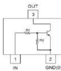
Device Schematic
