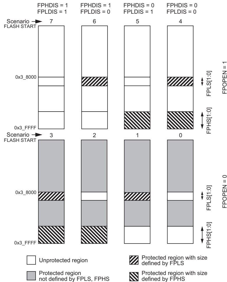
Figure 106. P-Flash Protection Scenarios
