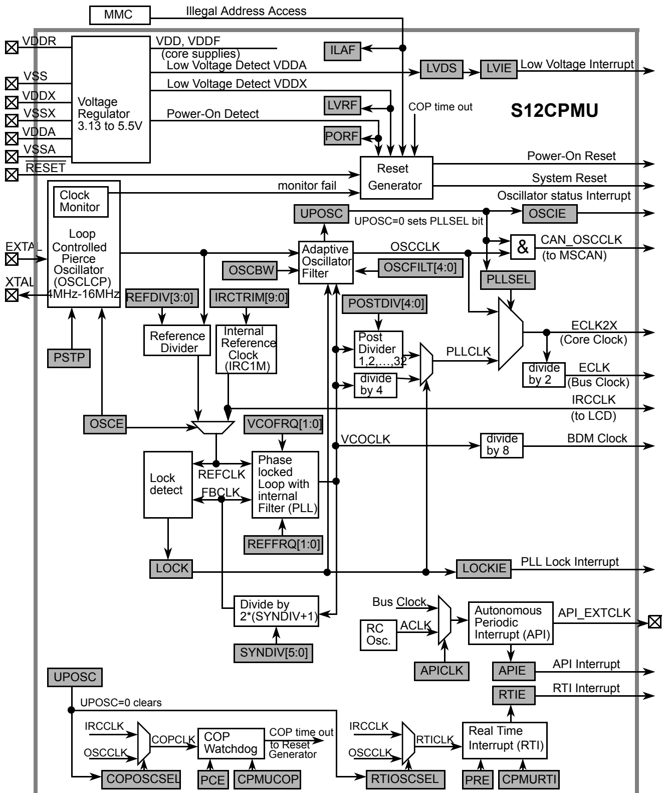
Figure 82. Block diagram of S12IPIMV1
