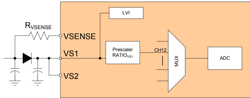
Figure 40. VS1Sense Module
