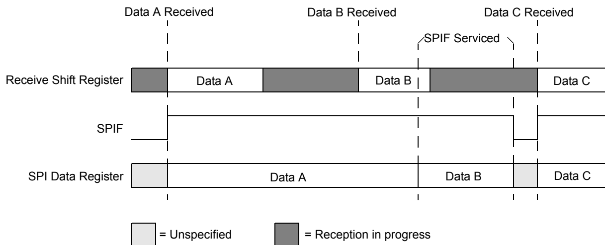
Figure 97. Reception with SPIF Serviced in Time
