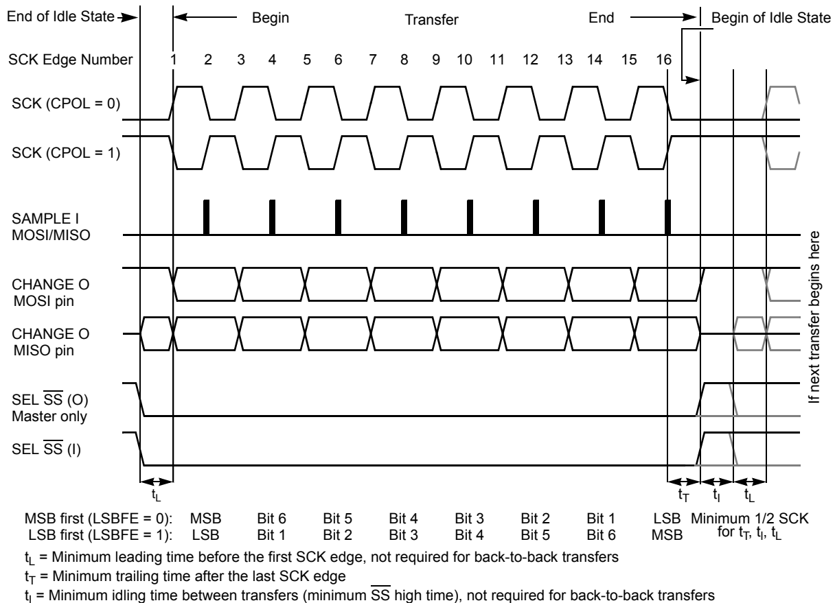
Figure 102. SPI Clock Format 1 (CPHA = 1), with 8-Bit Transfer Width Selected (XFRW = 0)
