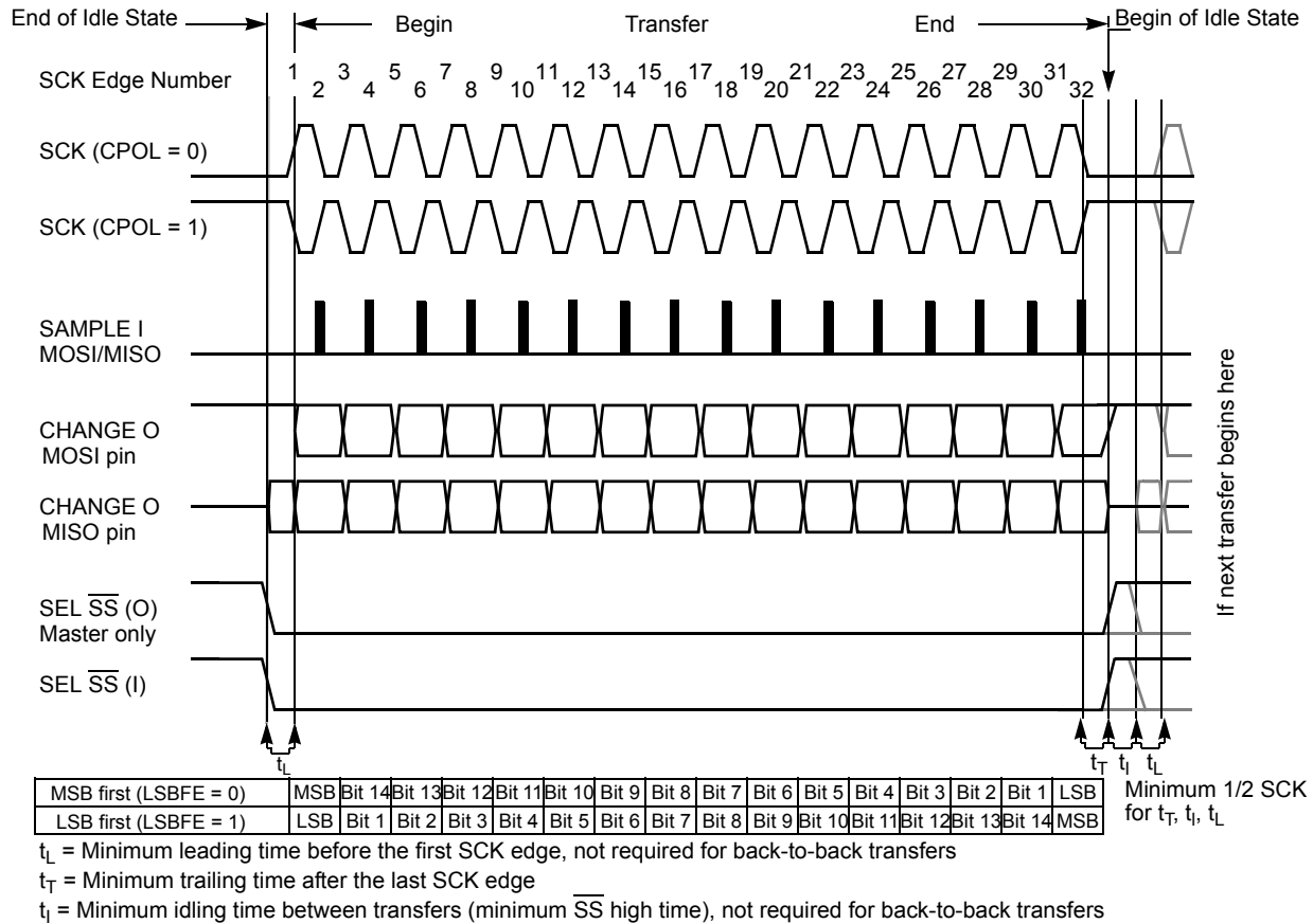
Figure 103. SPI Clock Format 1 (CPHA = 1), with 16-Bit Transfer Width Selected (XFRW = 1)
