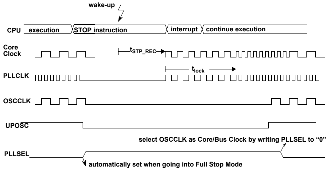
Figure 89. Full Stop Mode Using Oscillator Clock as Bus Clock
