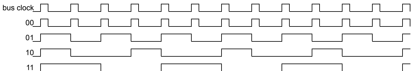
Figure 111. Interface Clock Waveforms for various D2DCLKDIV Encoding
