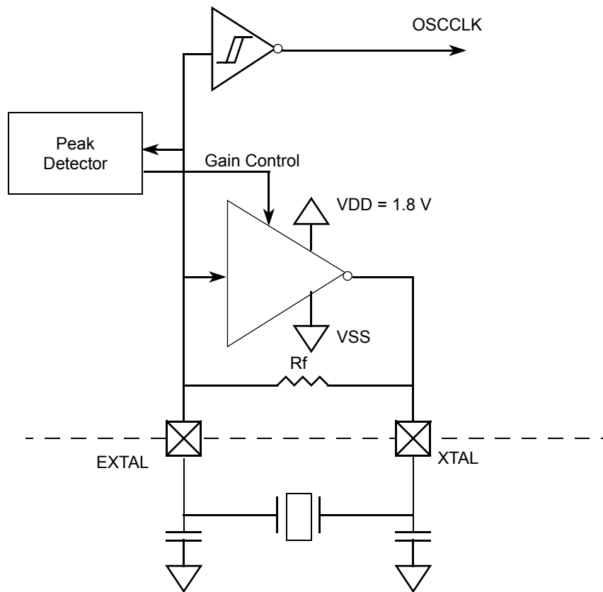
Figure 83. OSCLCP Block Diagram
