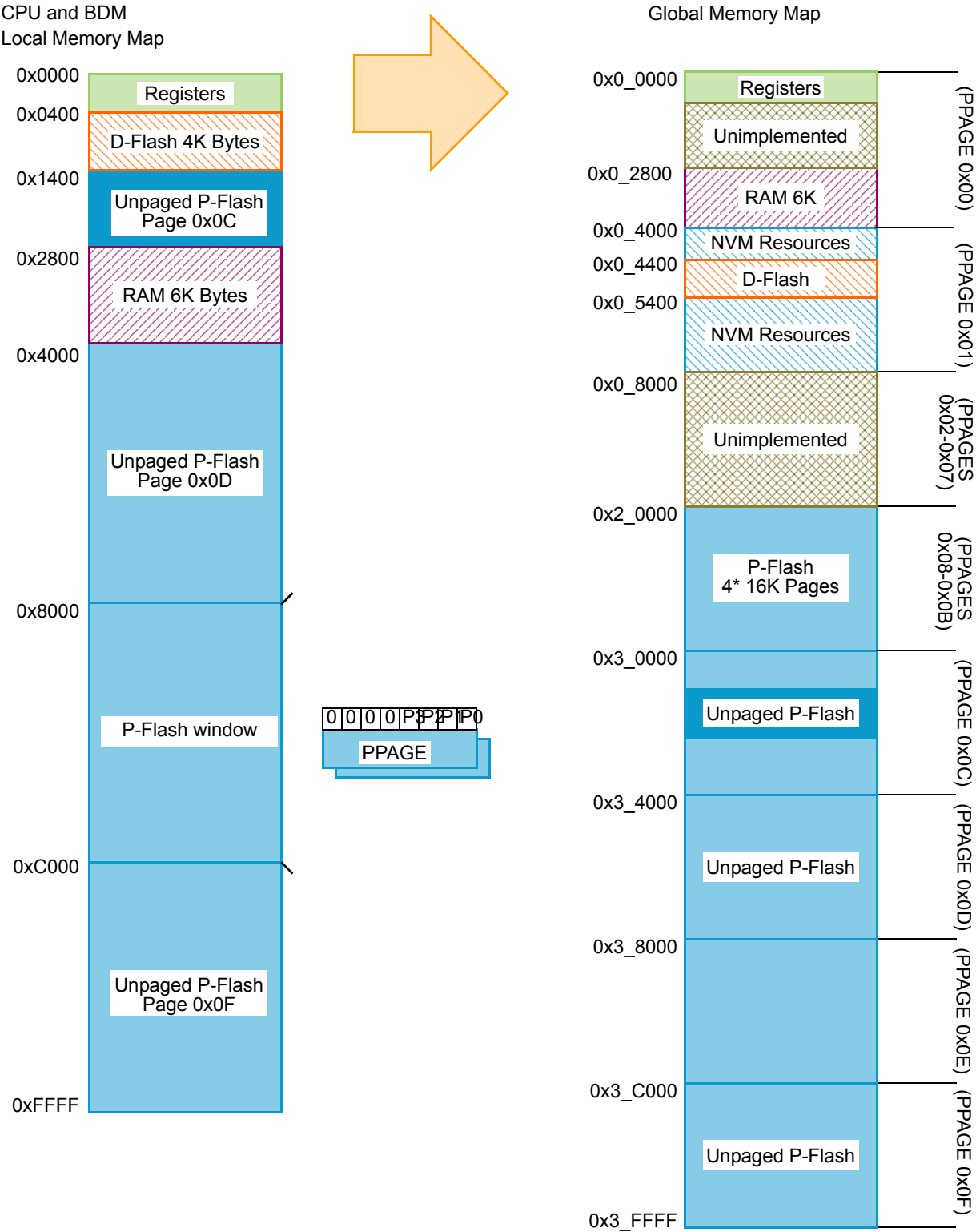
Figure 41. 9S121128 Global Memory Map
