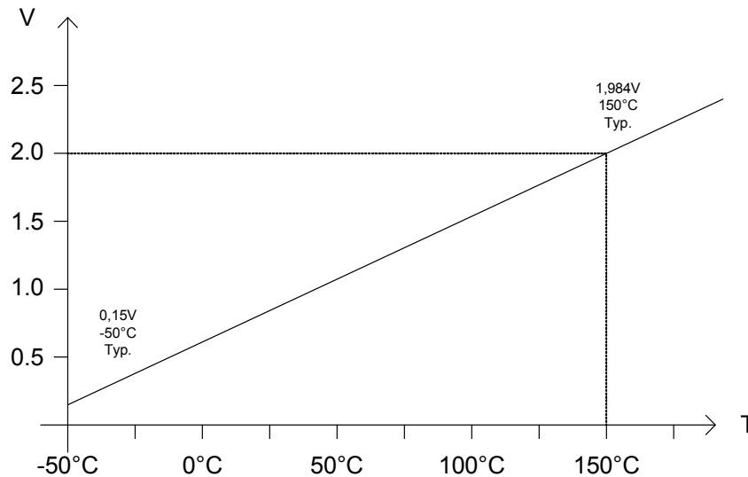
Figure 38. TSENSE - Graph
