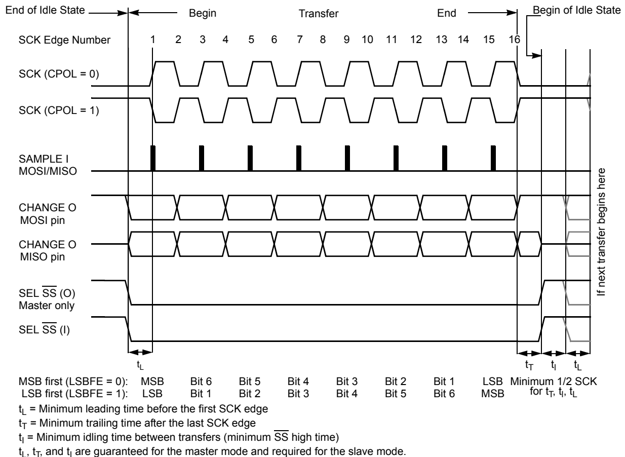
Figure 100. SPI Clock Format 0 (CPHA = 0), with 8-bit Transfer Width Selected (XFRW = 0)
