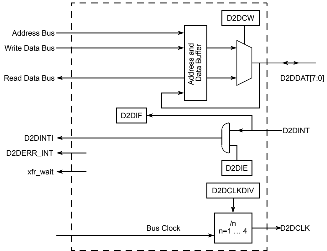
Figure 109. Die-to-Die Initiator (D2DI) Block Diagram
