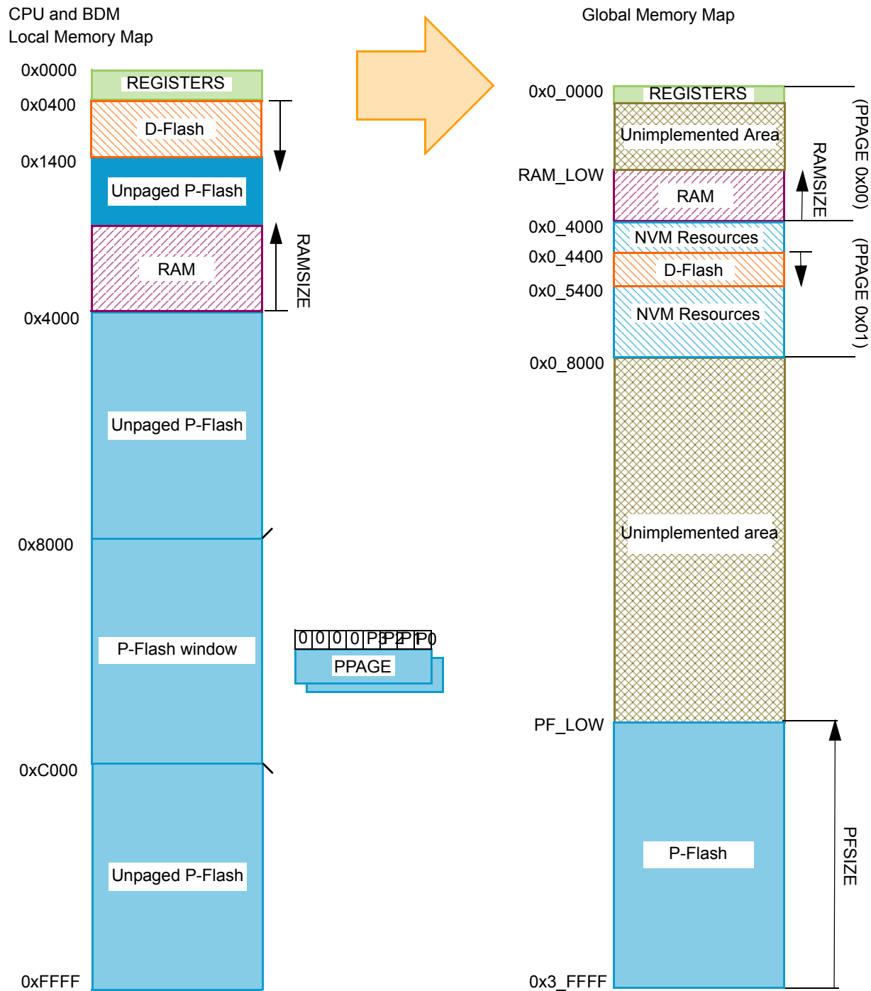
Figure 50. Implemented Global Address Mapping
