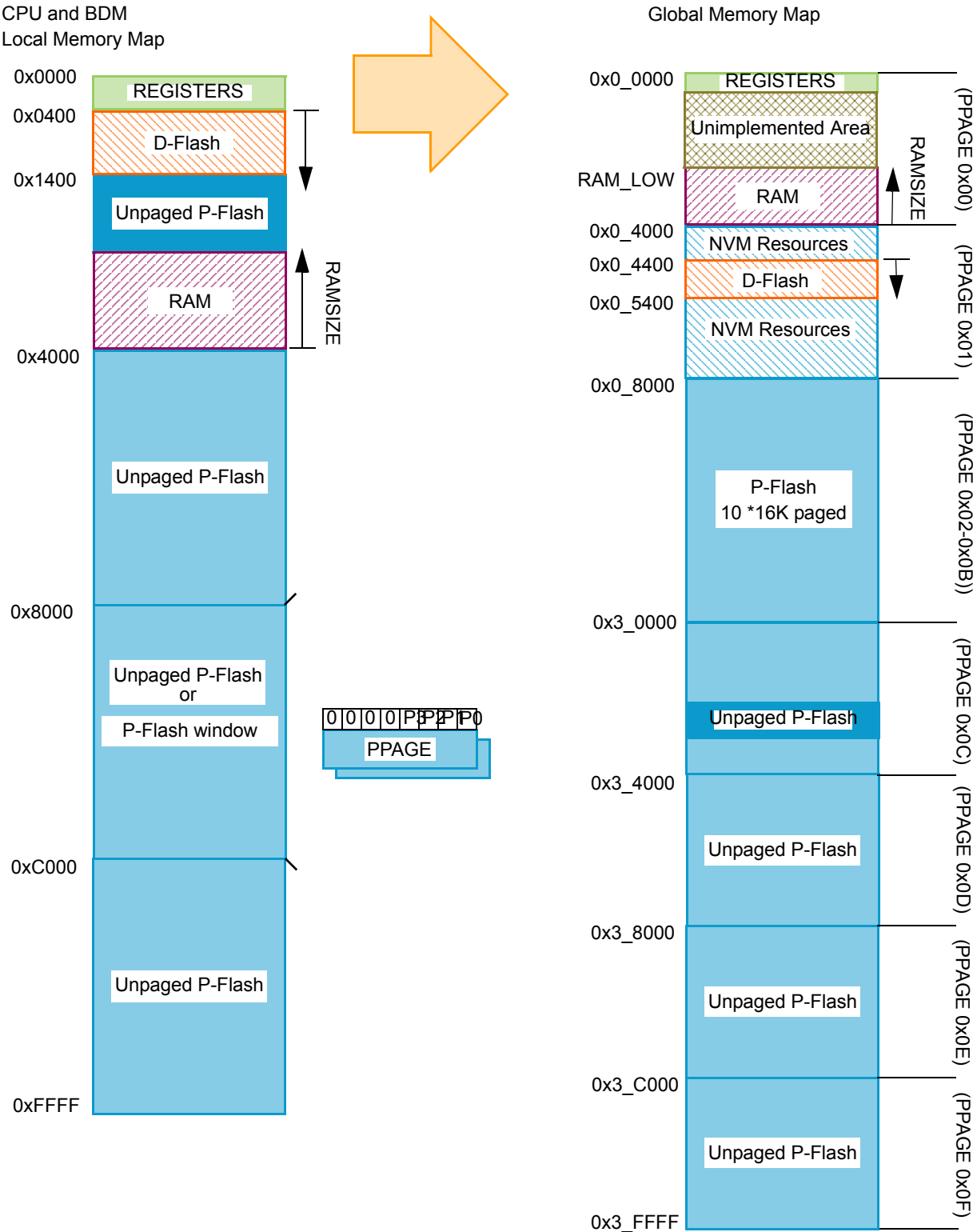
Figure 49. Local to Global Address Mapping
