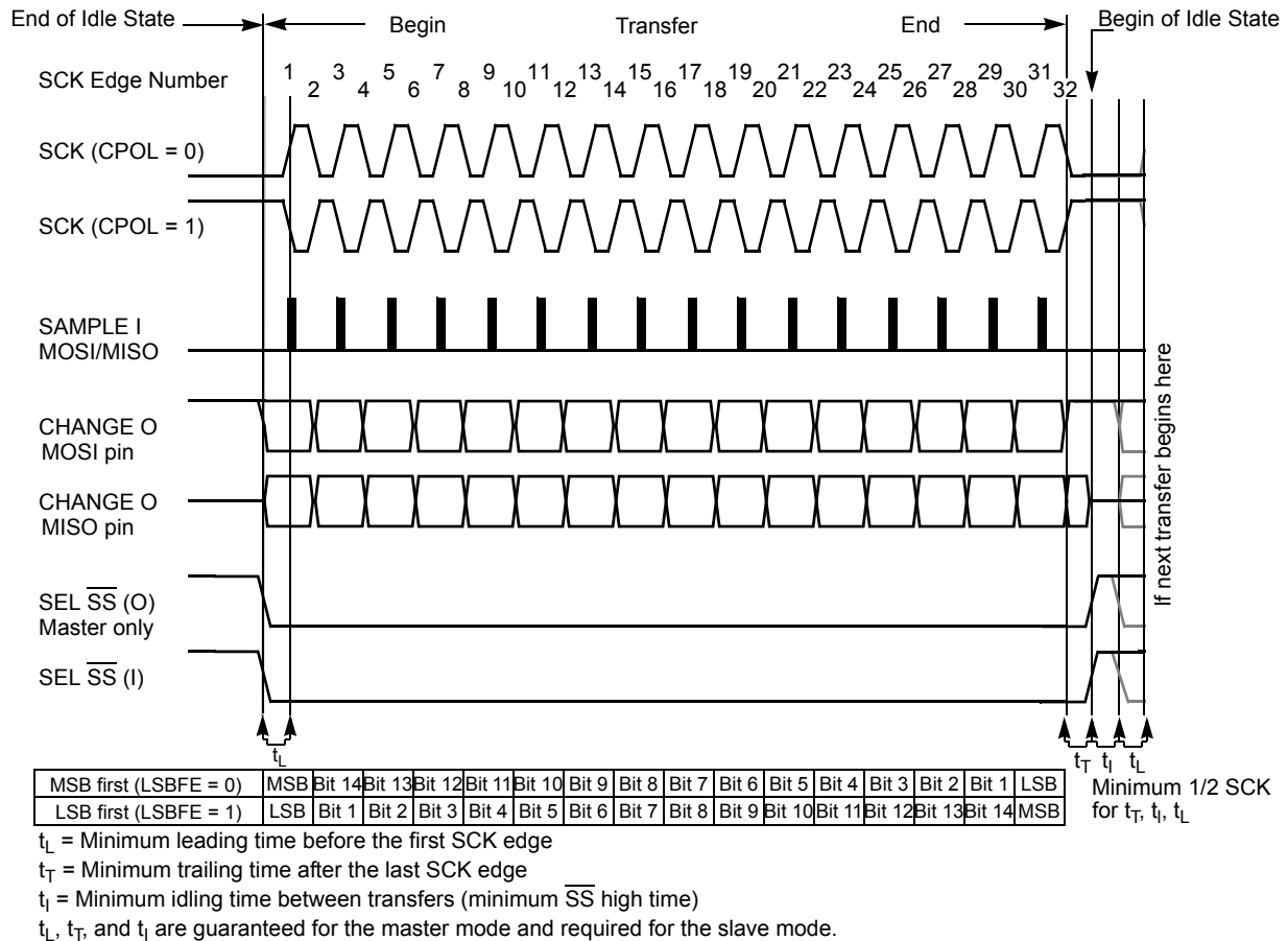
Figure 101. SPI Clock Format 0 (CPHA = 0), with 16-Bit Transfer Width Selected (XFRW = 1)
