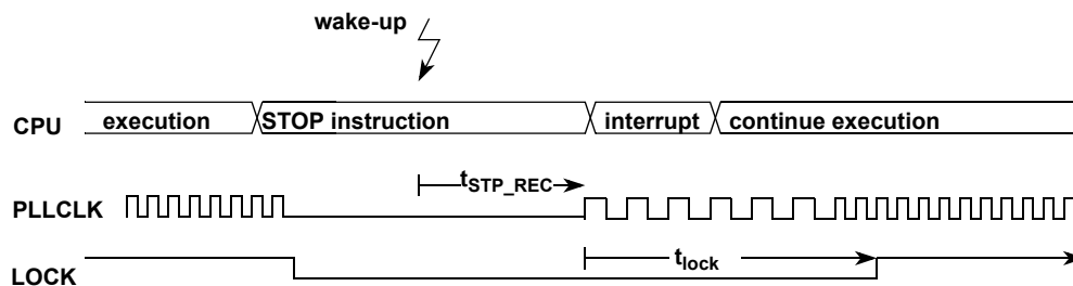
Figure 88. Stop Mode Using PLLCLK as Bus Clock
