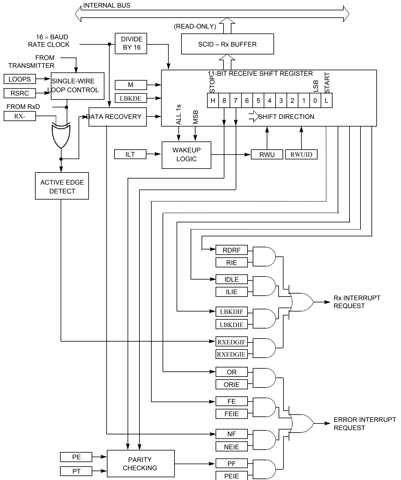
Figure 30. SCI Receiver Block Diagram
