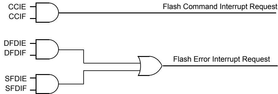
Figure 108. Flash Module Interrupts Implementation
