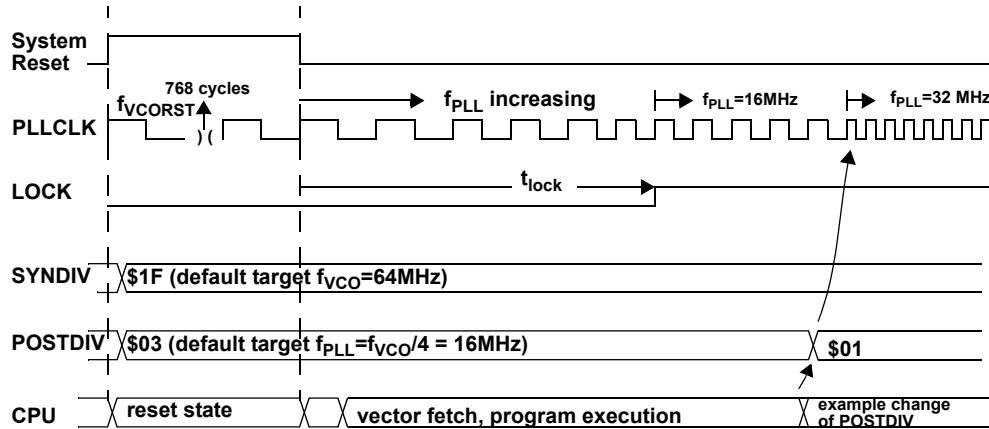
Figure 87. Startup of Clock System After Reset
