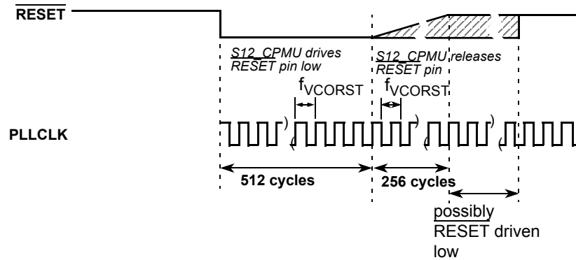
Figure 93. RESET Timing
