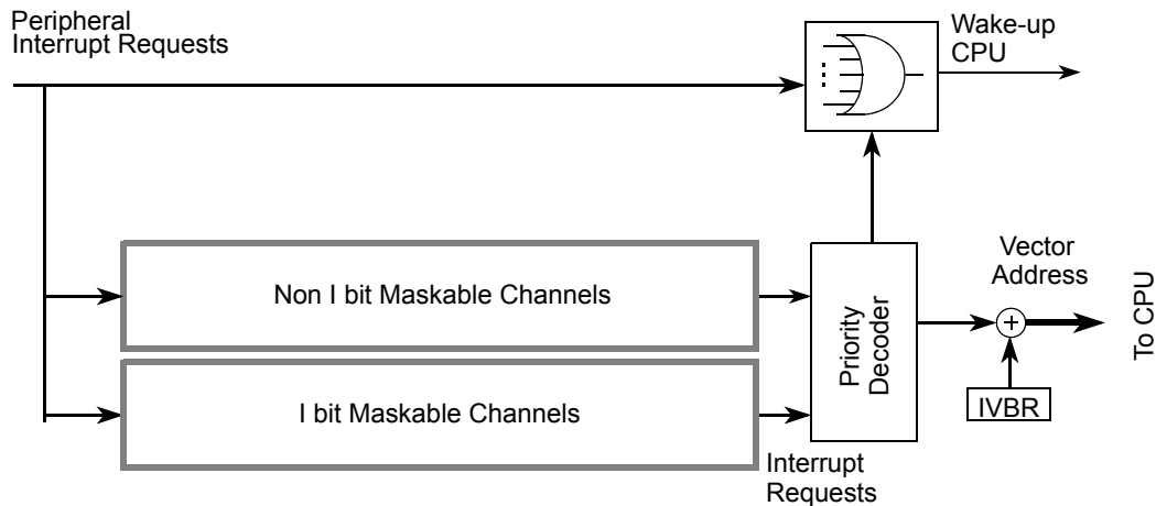
Figure 52. S12IPIMV1 Block Diagram
