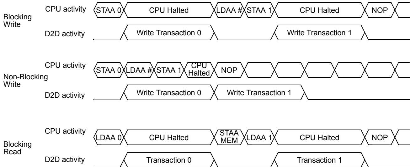
Figure 112. Blocking and Non-Blocking Transfers.
