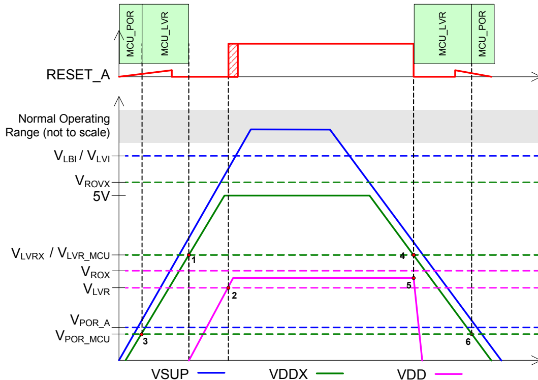
Figure 18. Power Up / Down Sequence
