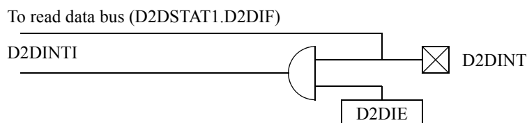
Figure 113. D2D External Interrupt Scheme
