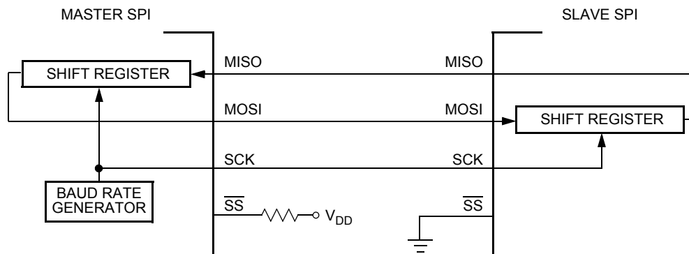
Figure 99. Master/Slave Transfer Block Diagram
