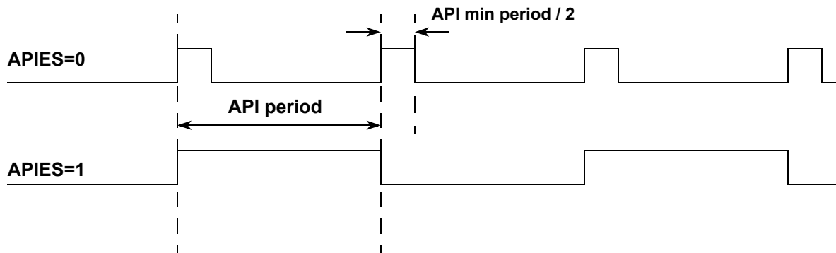
Figure 84. Waveform selected on API_EXTCLK pin (APIEA=1, APIFE=1)
