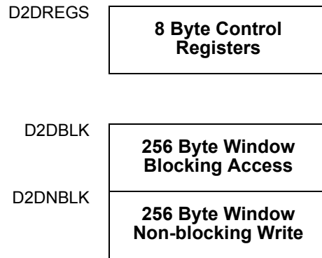
Figure 110. D2DI Top Level Memory Map
