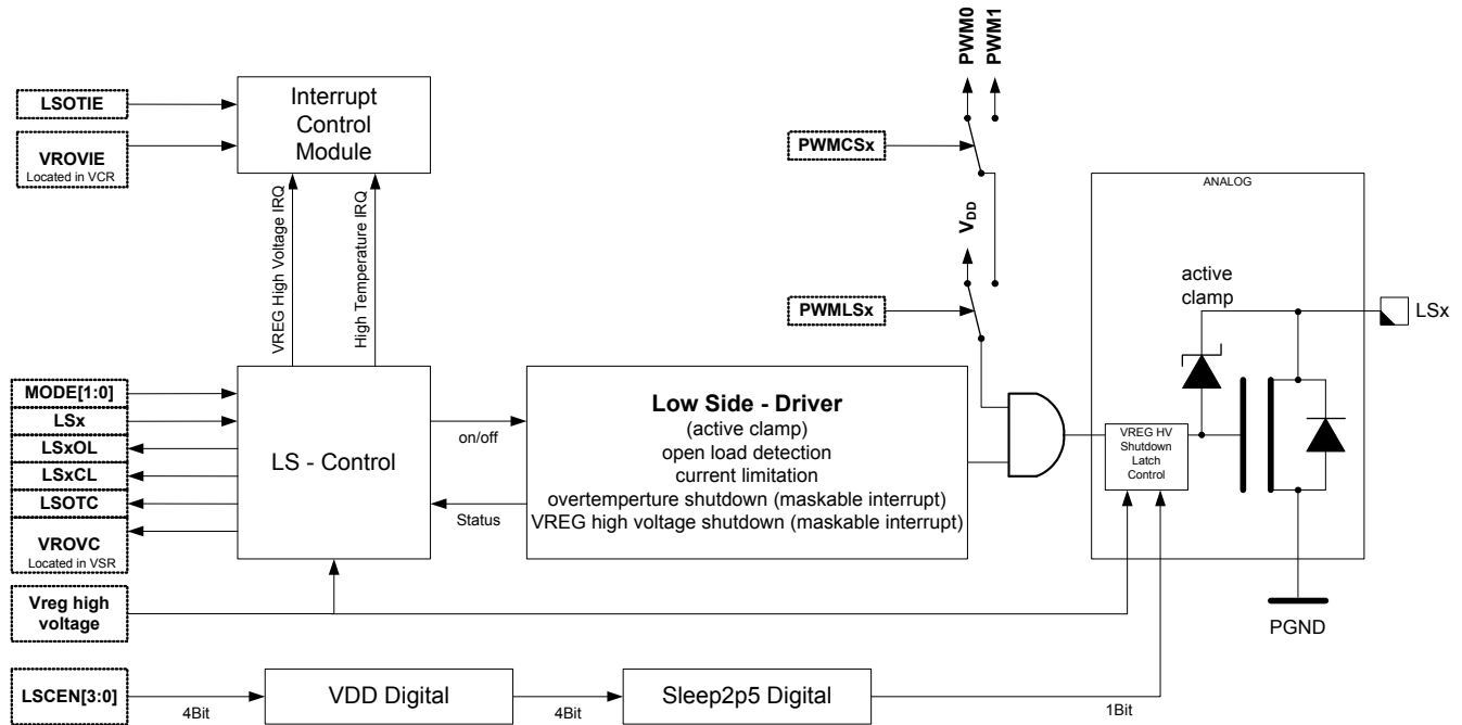
Figure 21. Low-side Drivers - Block Diagram
