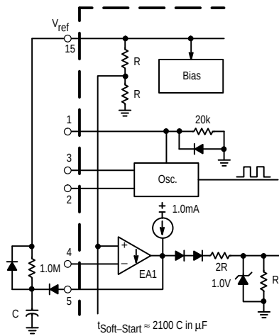
Figure 20. Soft-Start Circuit
