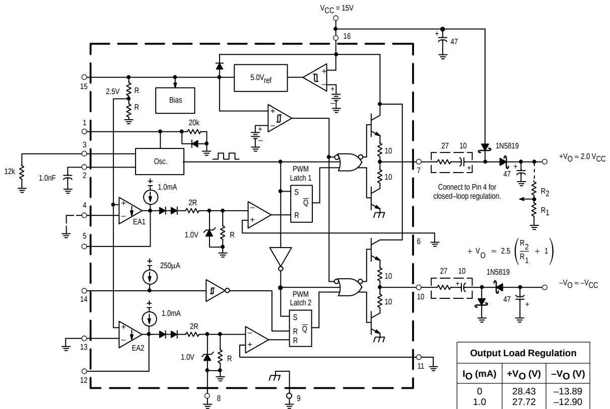
Figure 27. Dual Charge Pump Converter
