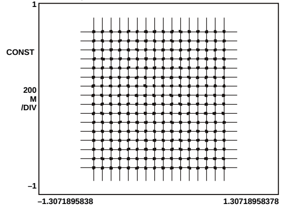
TRACE A: CH 1 256QAM MEAS TIME
