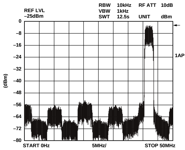
Figure 3. QPSK at 42 MHz and 2.56 MS/sec; 10.24 MHz External Clock with REFCLK Multiplier = 12, CIC = 3, HB3 On, 2x Data
