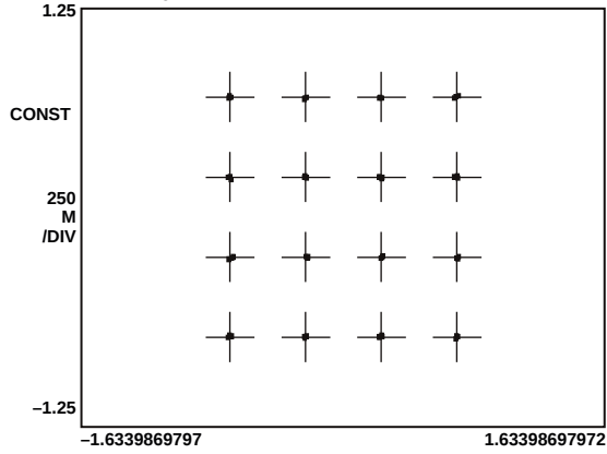
TRACE A: CH 1 16QAM MEAS TIME
