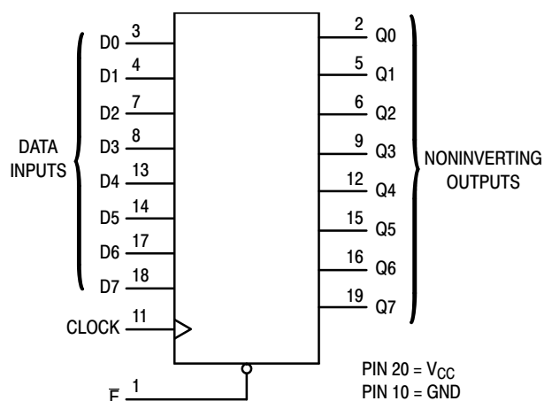
Figure 1. Logic Diagram
